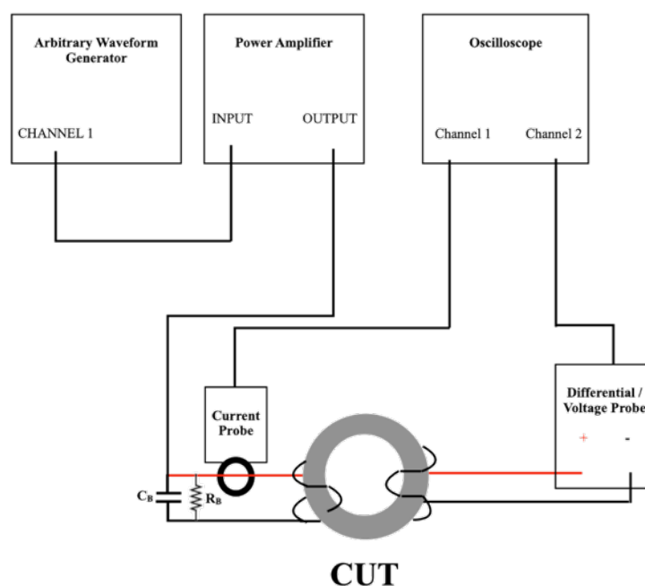
Core Loss Testing - Low Voltage with Amplifier. Typical Test Setup: System Block Diagram.
