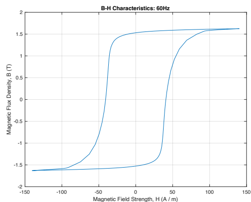
100°C. Sample Sinusoidal Excitation Waveform and B-H Plot. 273.00 mV pp 60Hz, Amplifier Gain X50.
