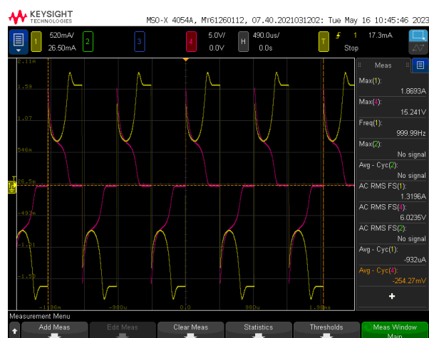
150°C. Sample Square Excitation Waveform and B-H Plot. 242.00 mV pp 1kHz, Amplifier Gain X50.
