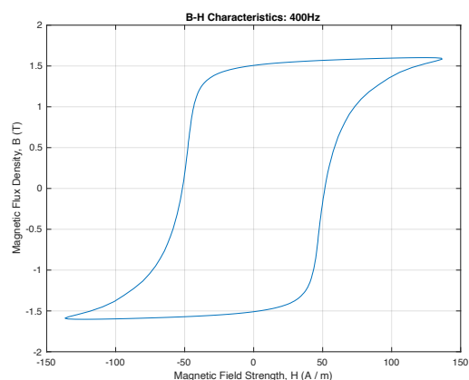
150°C. Sample Triangular Excitation Waveform and B-H Plot. 278 mV pp 400Hz, Amplifier Gain X50.
