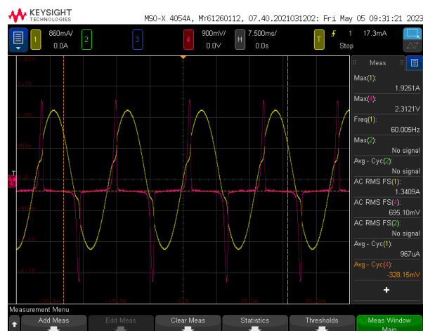
100°C. Sample Sinusoidal Excitation Waveform and B-H Plot. 273.00 mV pp 60Hz, Amplifier Gain X50.
