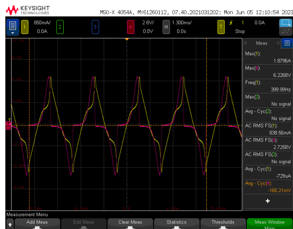
150°C. Sample Triangular Excitation Waveform and B-H Plot. 278 mV pp 400Hz, Amplifier Gain X50.
