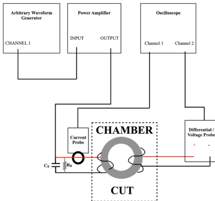
Core Loss Testing - Low Voltage with Amplifier. Typical Test Setup: System Block Diagram.
