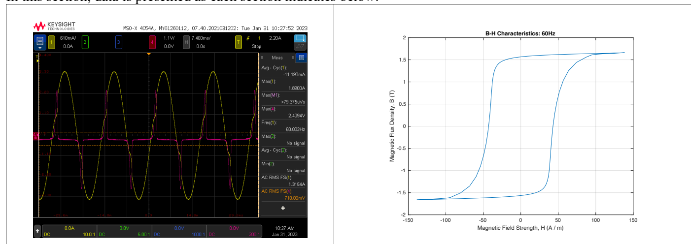
Sample Sinusoidal Excitation Waveform and B-H Plot. Sinusoidal Signal. 273.00 mV pp 60Hz, Amplifier Gain X50.
