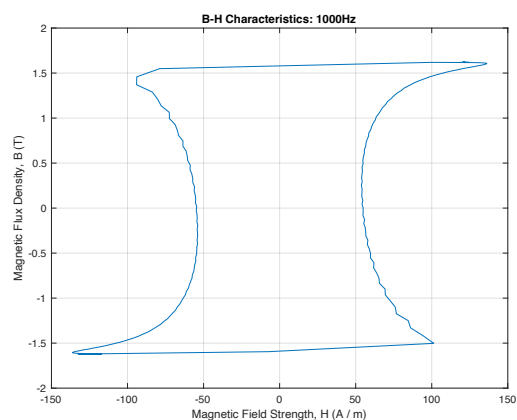
150°C. Sample Square Excitation Waveform and B-H Plot. 242.00 mV pp 1kHz, Amplifier Gain X50.
