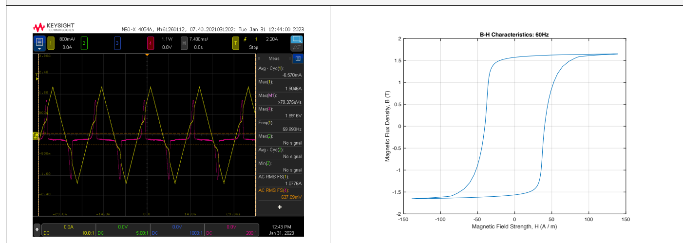
Sample Triangular Excitation Waveform and B-H Plot. Triangular Signal. 274.00 mV pp 60Hz, Amplifier Gain X50.
