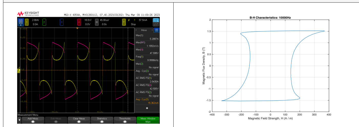
Sample Square Excitation Waveform and B-H Plot. Square Signal. 1.005 V pp 10kHz, Amplifier Gain X50.
